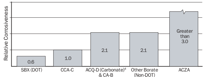
Note: The above data are based on accelerated testing per AWPA Standard E12-94, and may or may not have a relation to actual service life.
